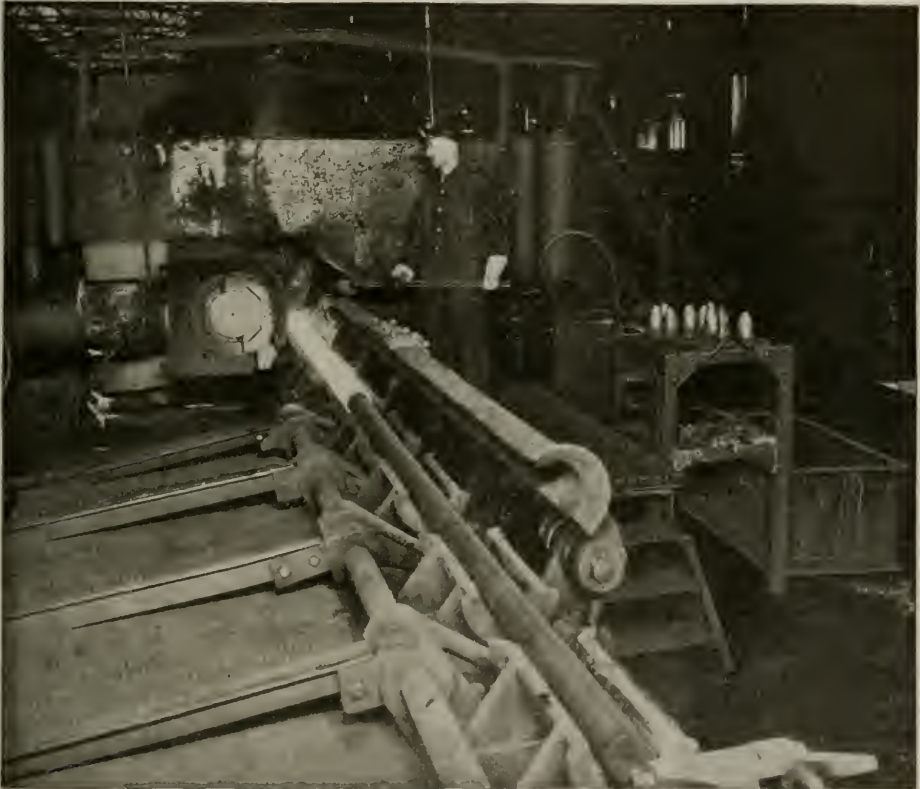
ROUGH TUBE COMING THROUGH PIERCING MILL
